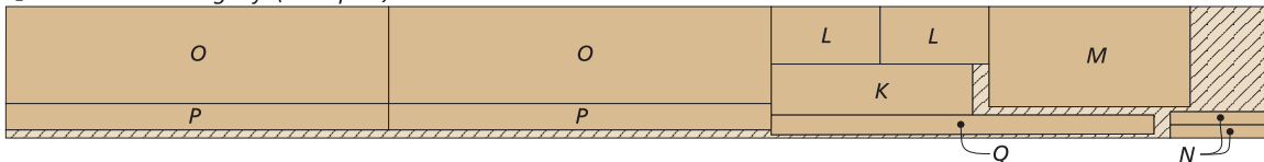
1\frac{3}{4} " x 5" - 48" Mahogany (3.3 Bd. Ft.)
